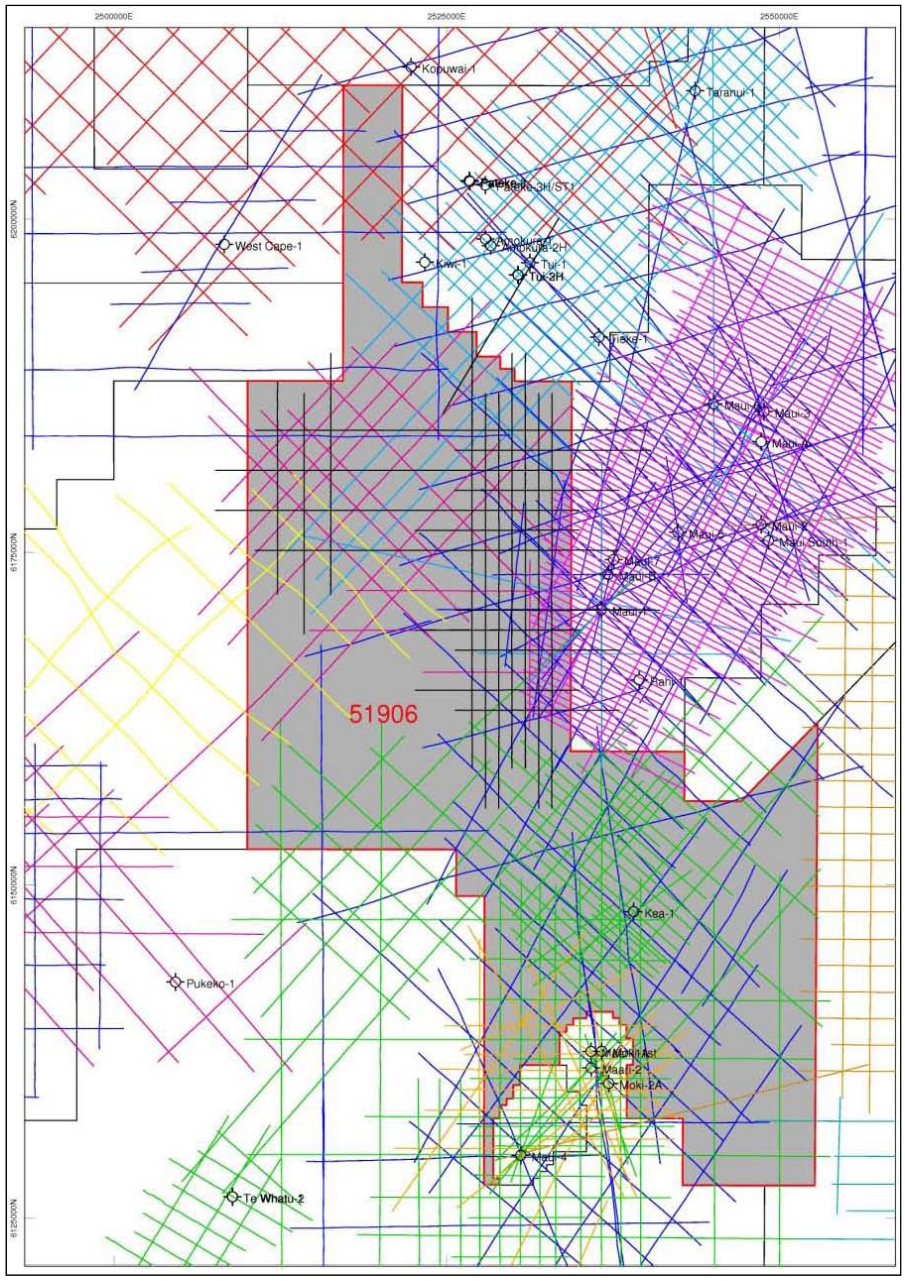
Existing 2D Seismic coverage in PEP51906
