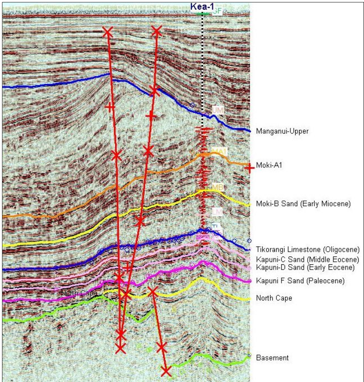
Seismic Section at Kea-1 Location
